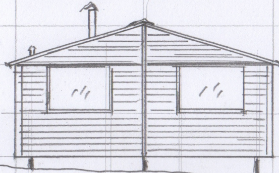
SOUTHWEST ELEVATION
